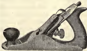
FIG. 5. SMOOTHER PLANE.
