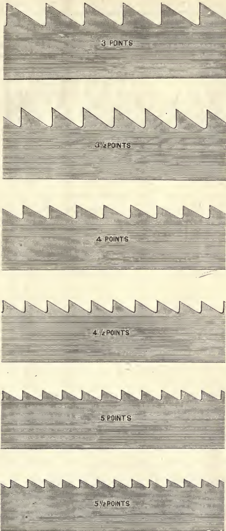
FIG. 1. RIP SAWS.
