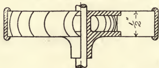
FIG. 5.—PLAN OF WHEEL.
