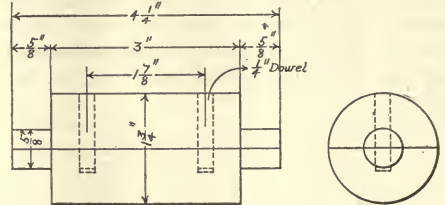
FIGS. 38 AND 39. CASTING AND SPLIT PATTERN FOR RECESSED CYLINDER.
