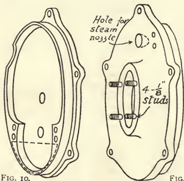
ENDS OF TURBINE CASING.
