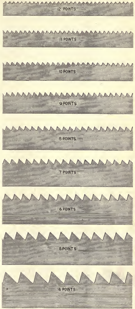
FIG. 2. CROSS-CUT SAWS.
