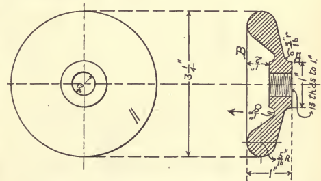
FIG. 14. HANDWHEEL.
