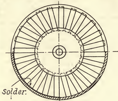
FIG. 4.—ELEVATION OF WHEEL.
