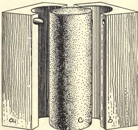
FIG. 23. CORE AND CORE BOX.
